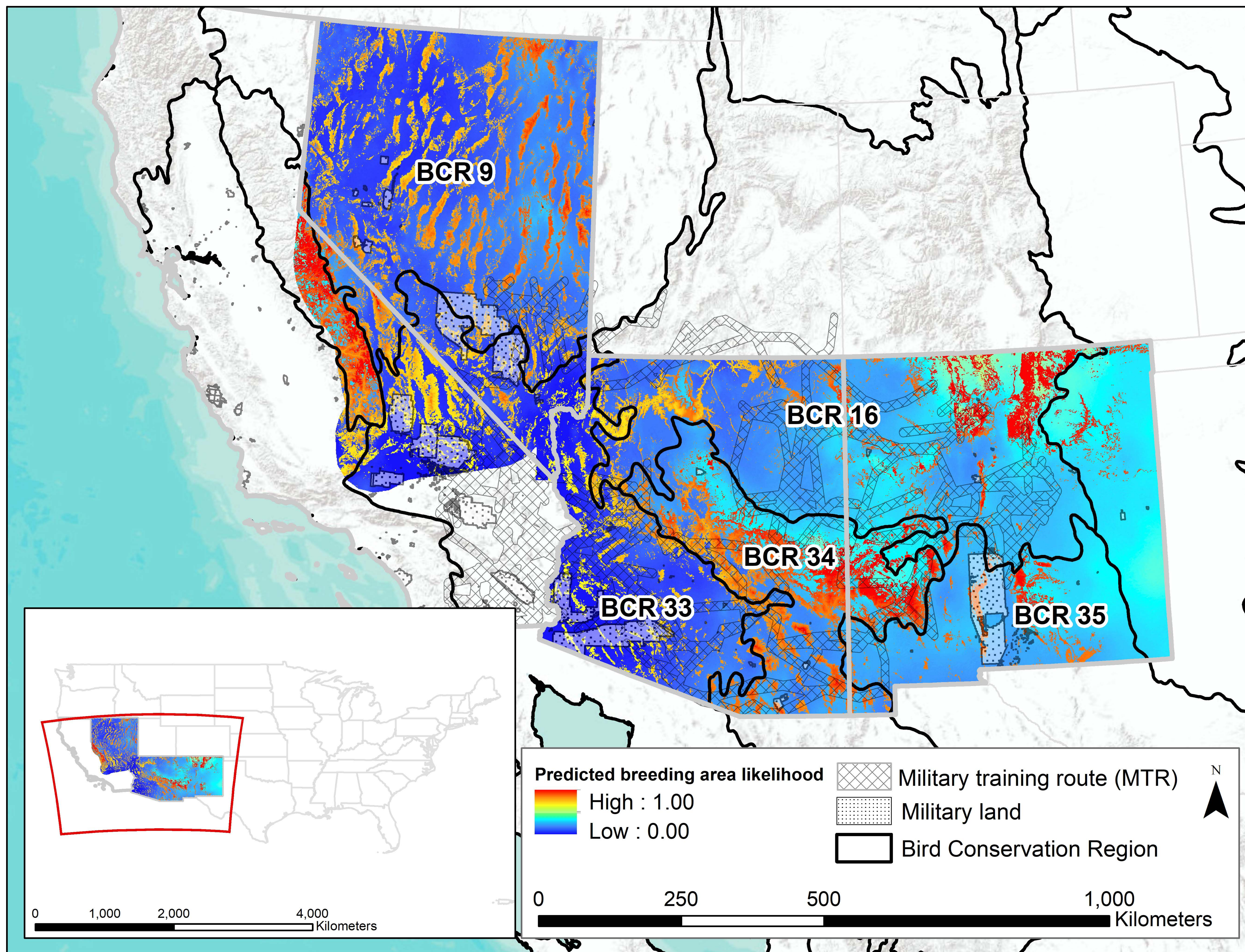
Predicted likelihood of golden eagle nesting habitat using our global logistic regression model based on 914 surveyed golden eagle nesting territories in the southwestern U.S. Locations symbolized as a dark red indicate areas with the highest predicted likelihood of golden eagle nesting habitat while those in a dark blue indicate the lowest likelihood.
